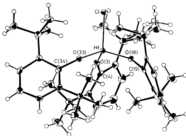
Figure 1. A view of the HfCl(OC_{14}H_{21})_3 molecule giving the atom numbering scheme used. Some pertinent bond distances and angles are: Hf(1)-Cl(2) = 2.365(1) , Hf(1)-O(3) = 1.938(3) , Hf(1)-O(18) = 1.925(2) , Hf(1)-O(33) = 1.917(3) Å, Cl(2)-Hf(1)-O(3) = 109.5 , Cl(2)-Hf(1)-O(18) = 103.9 , Cl(2)-Hf(1)-O(33) = 108.8 , O(3)-Hf(1)-O(18) = 114.9 , O(3)-Hf(1)-O(33) = 109.9 , O(18)-Hf(1)-O(33) = 109.7 , Hf(1)-O(3)-C(4) = 159.4 , Hf(1)-O(18)-C(19) = 152.0 , Hf(1)-O(33)-C(34) = 155.9^\circ .
